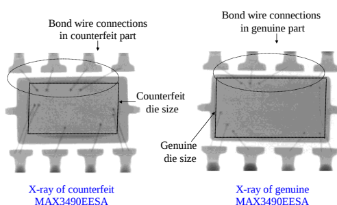
Figure 2: Example of X-ray inspection 6
